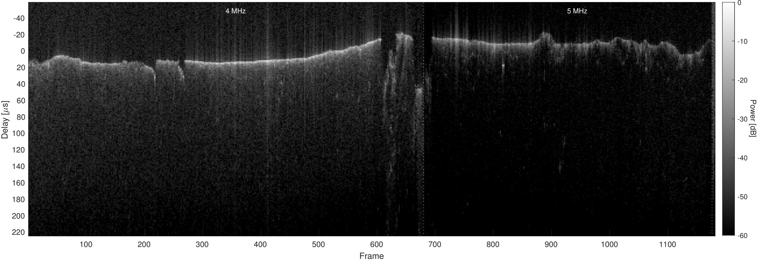
Orbit 9242, Optimized, No Window, Channel 2
