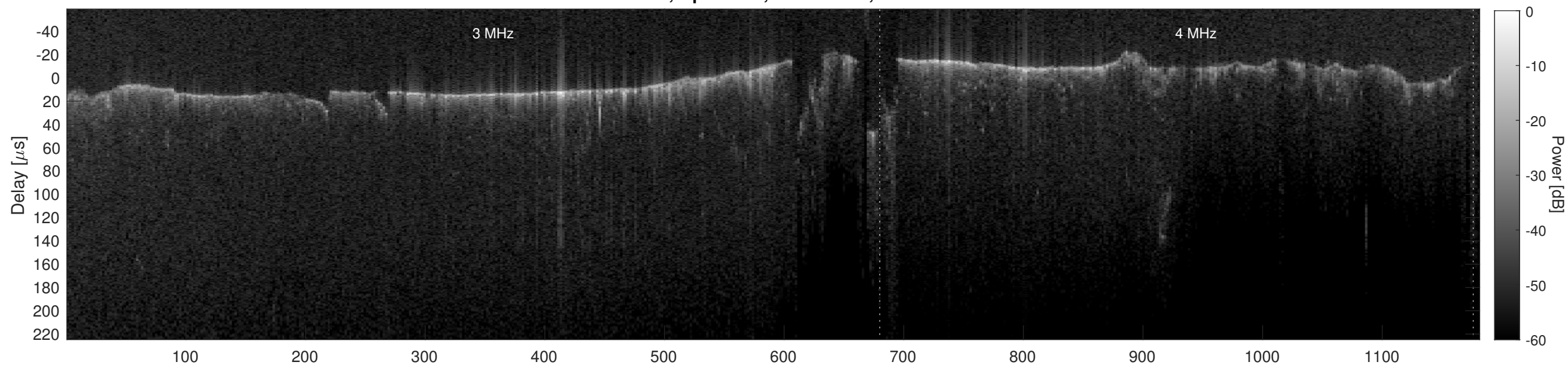
Orbit 9242, Cluttergram
