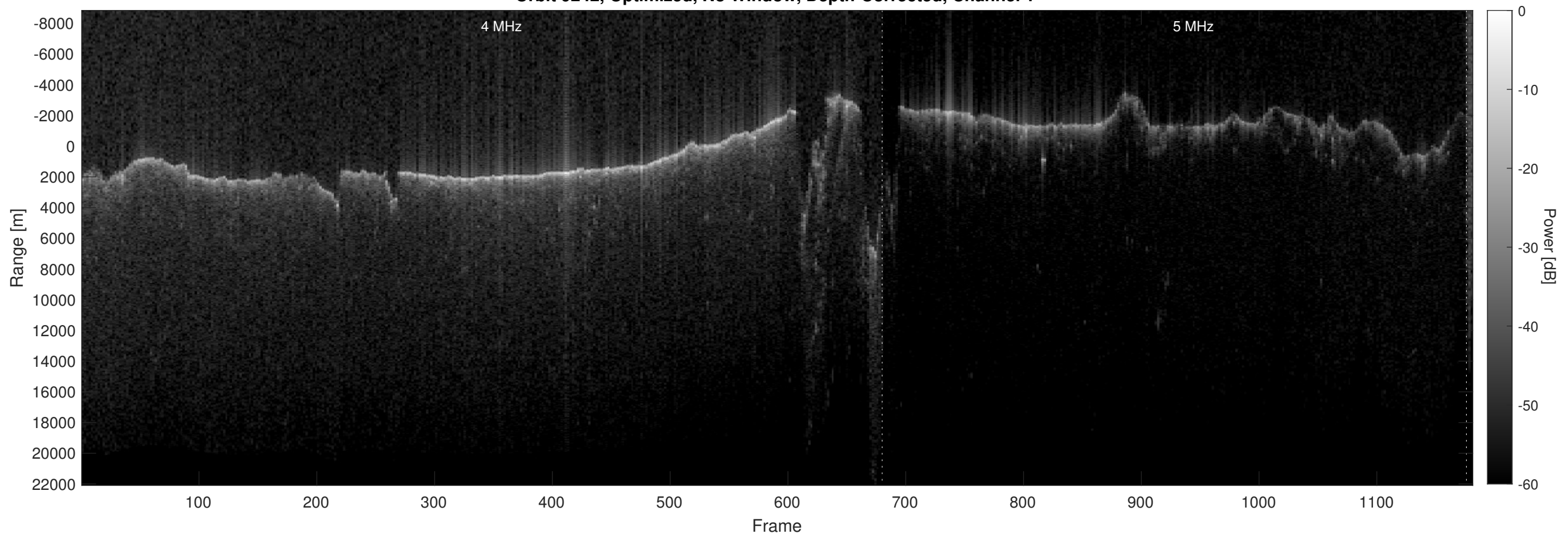
Orbit 9242, Optimized, No Window, Depth-Corrected, Channel 2
