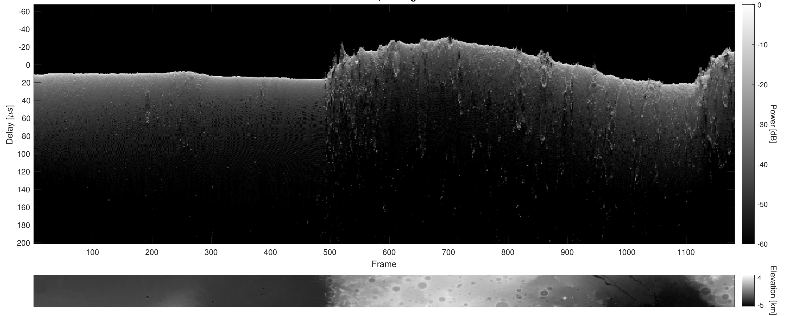
Orbit 9244, Cluttergram
