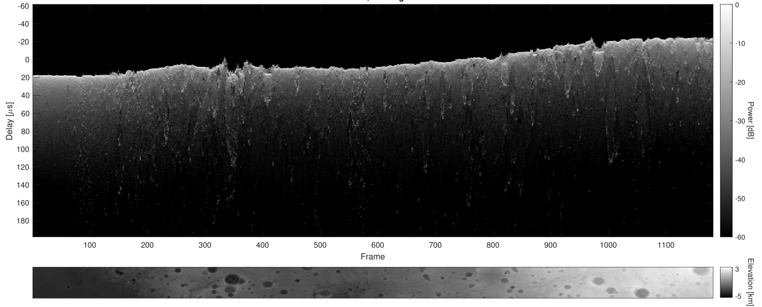
Orbit 9245, Cluttergram
