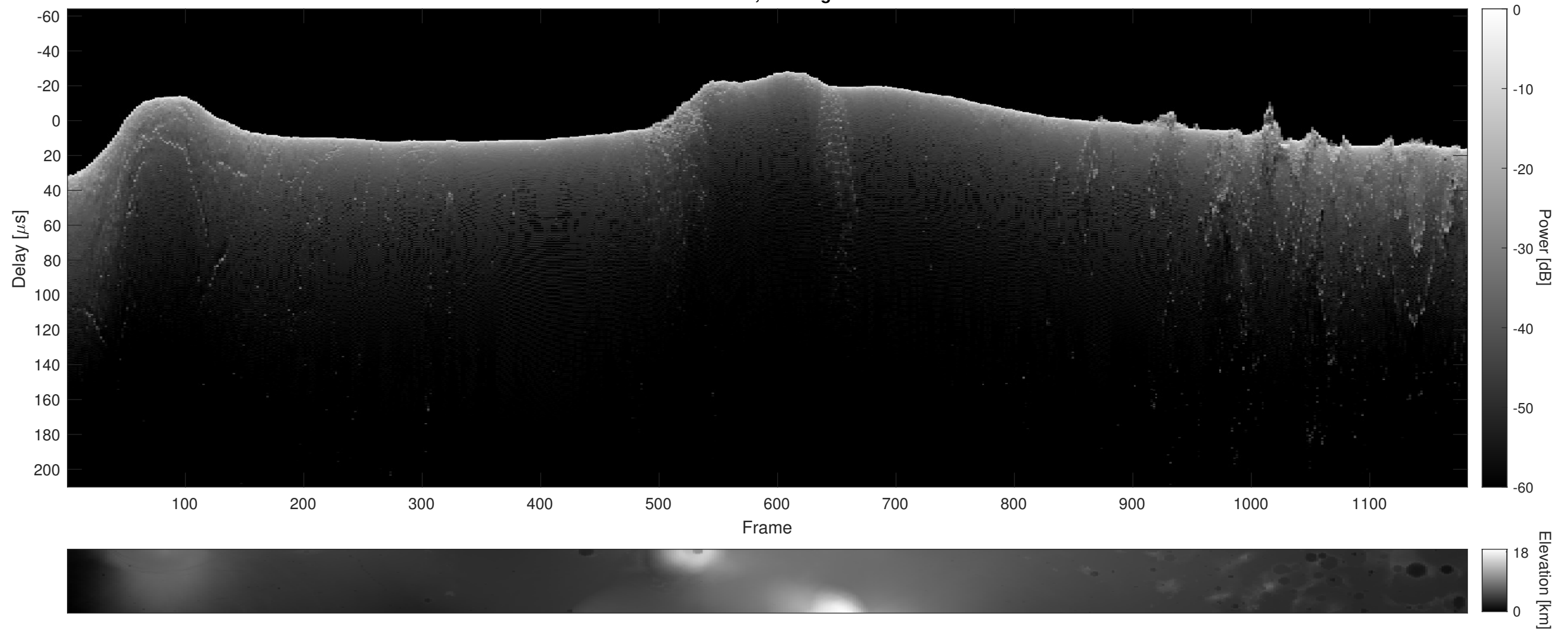
Orbit 9246, Cluttergram
