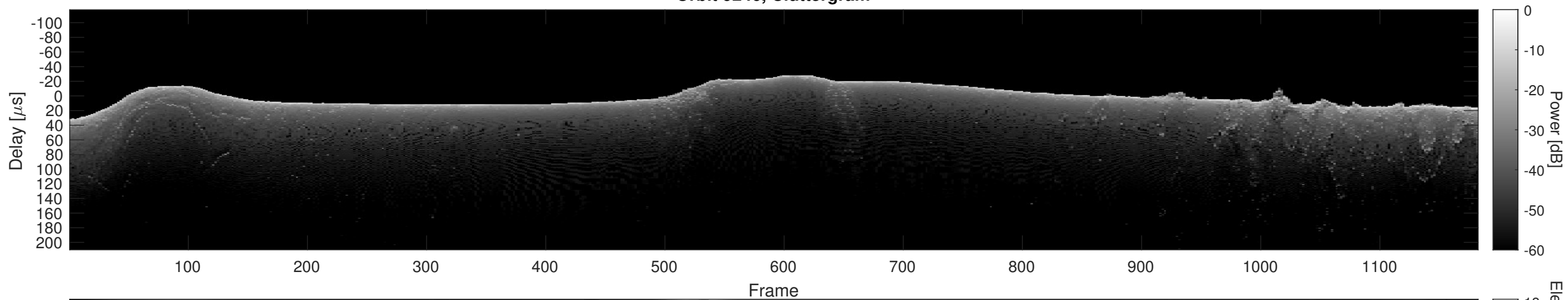
Orbit 9246, Cluttergram
