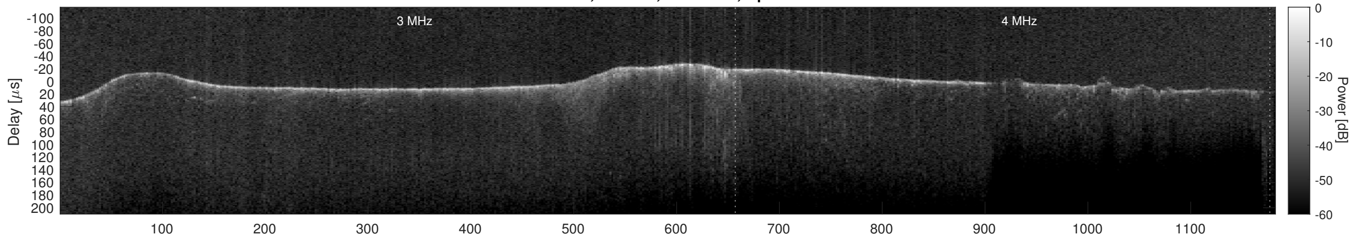
Orbit 9246, Cluttergram
