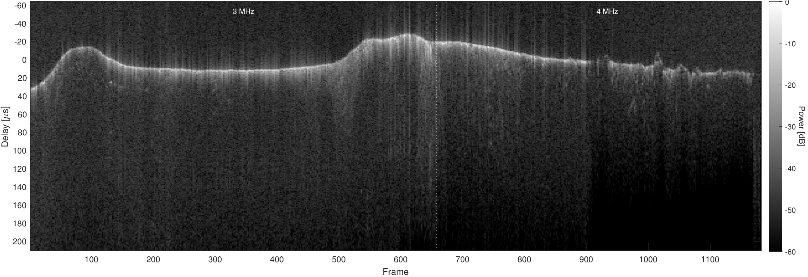
Orbit 9246, Optimized, No Window, Channel 2
