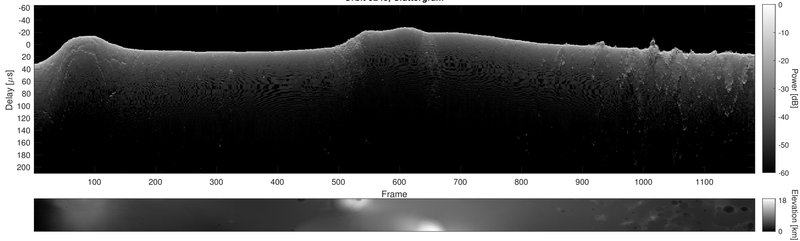
Orbit 9246, Cluttergram
