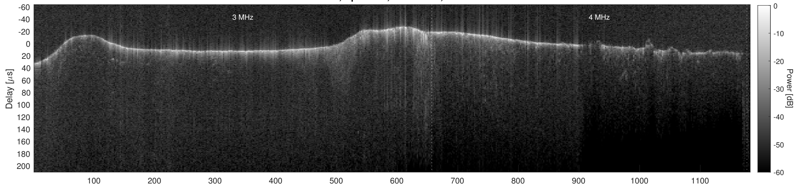
Orbit 9246, Cluttergram
