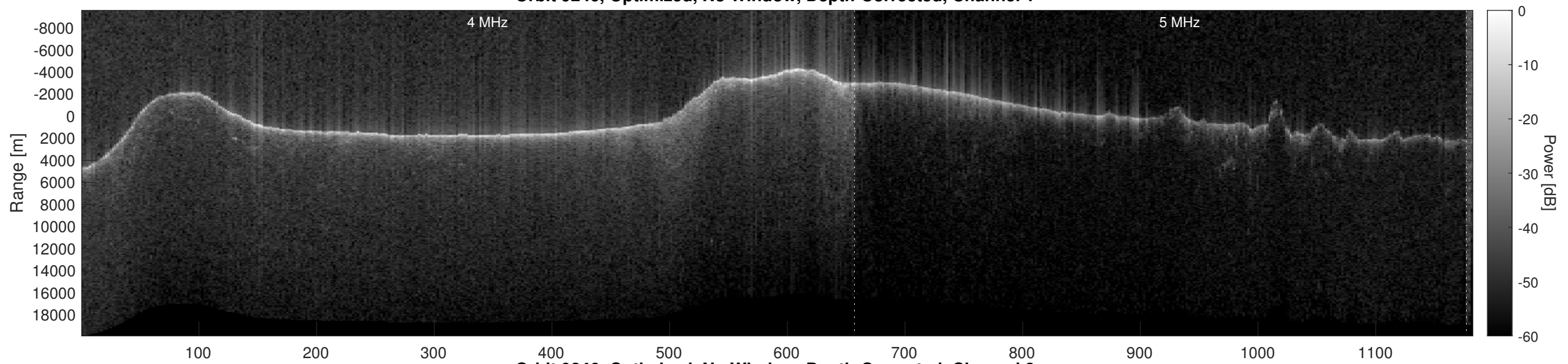
Orbit 9246, Optimized, No Window, Depth-Corrected, Channel 2
