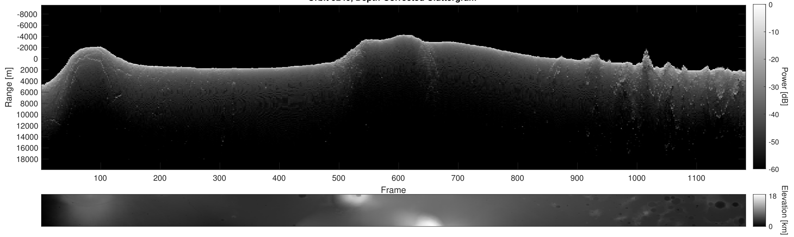
Orbit 9246, Depth-Corrected Cluttergram
