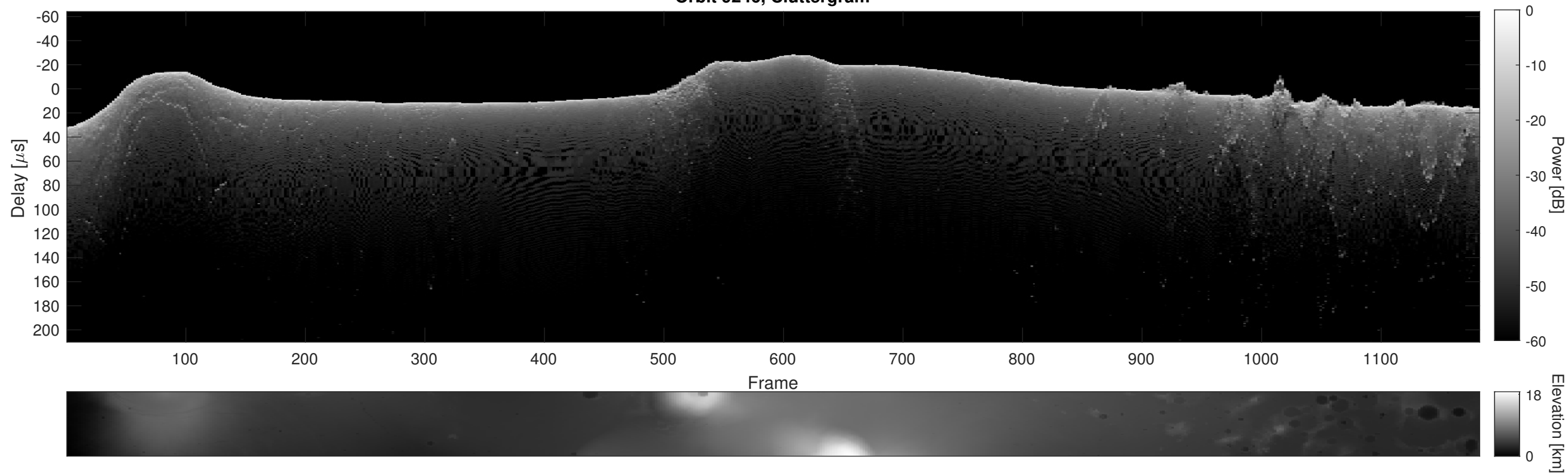
Orbit 9246, Cluttergram
