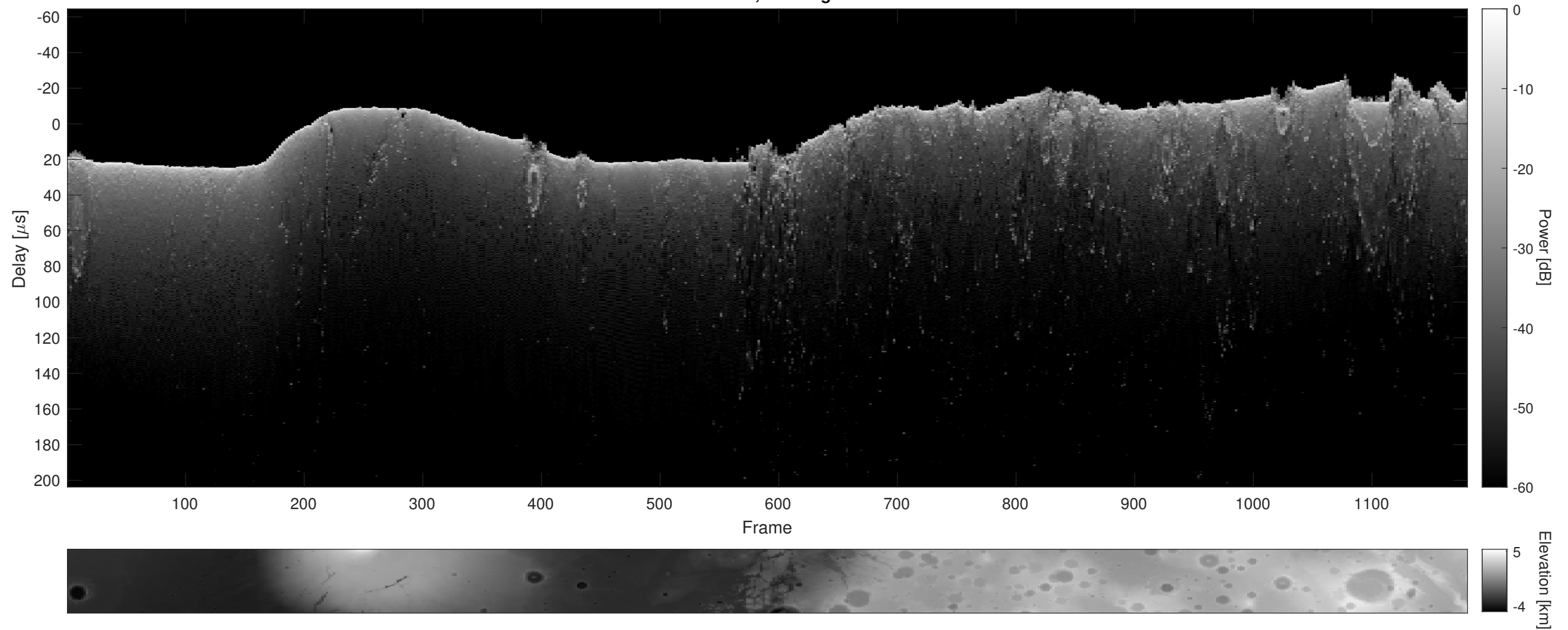
Orbit 9247, Cluttergram
