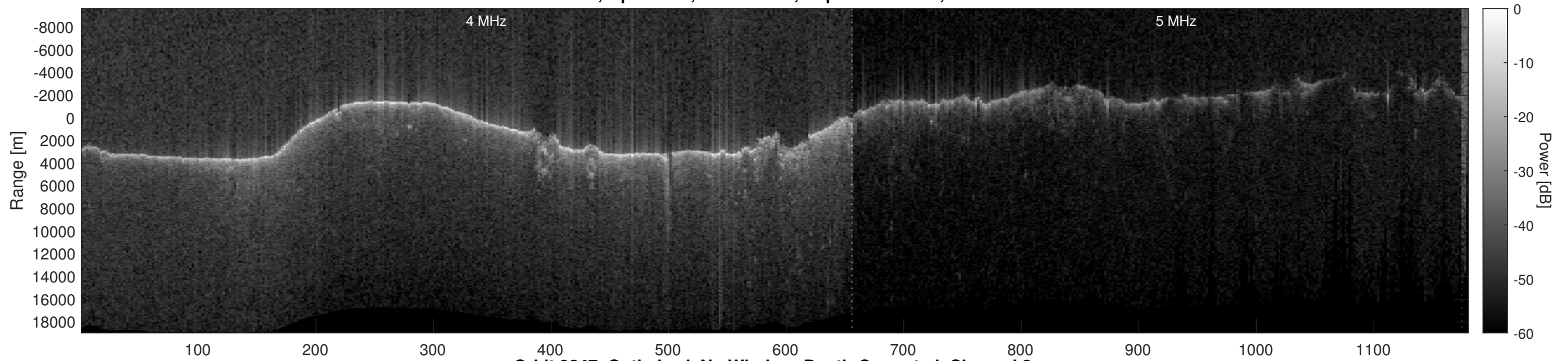
Orbit 9247, Optimized, No Window, Depth-Corrected, Channel 2
