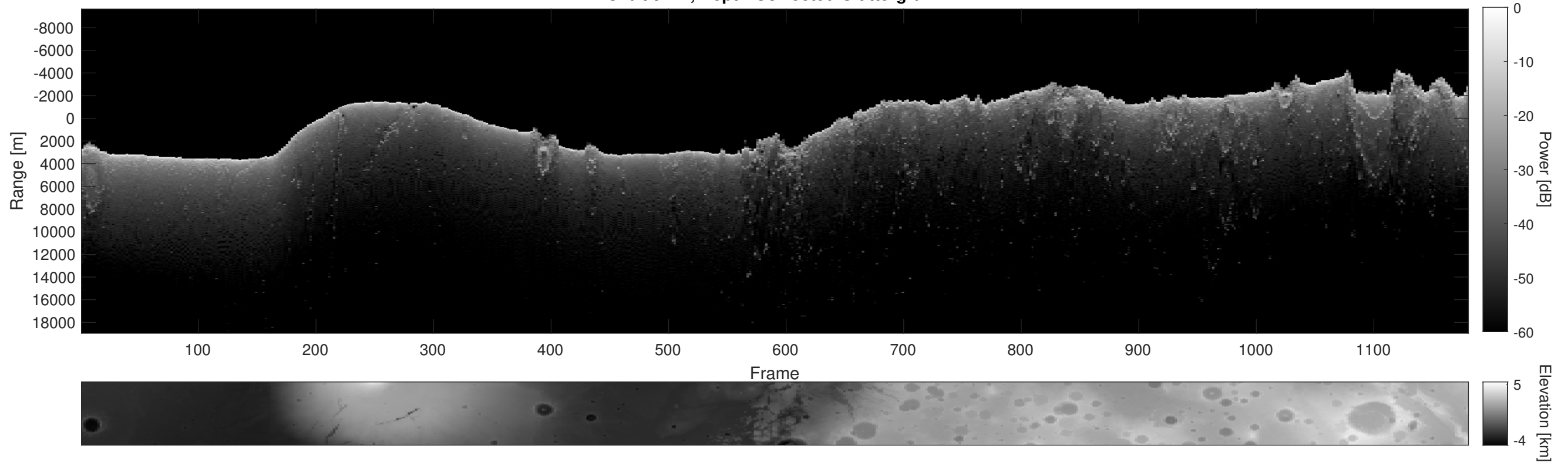
Orbit 9247, Depth-Corrected Cluttergram
