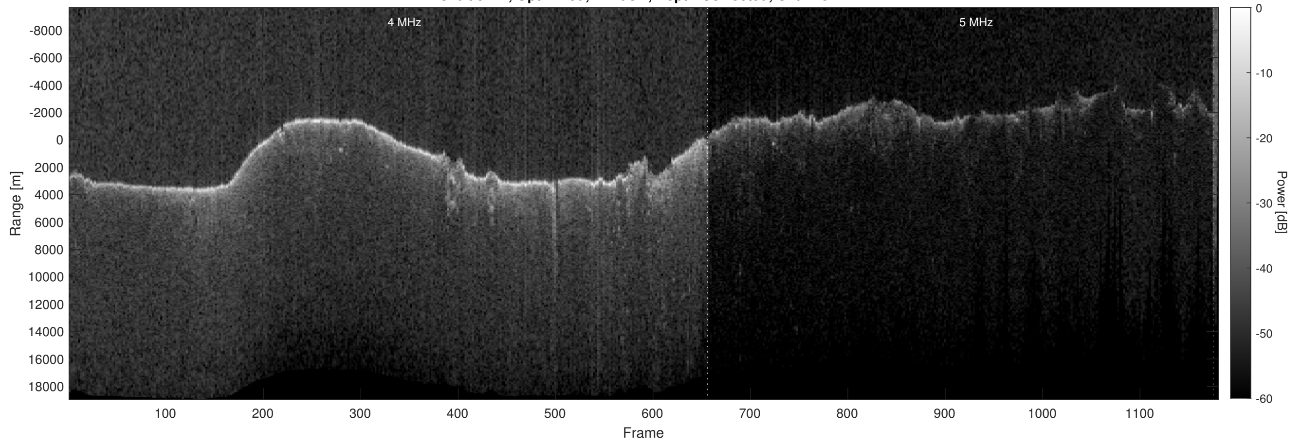
Orbit 9247, Optimized, Window, Depth-Corrected, Channel 2
