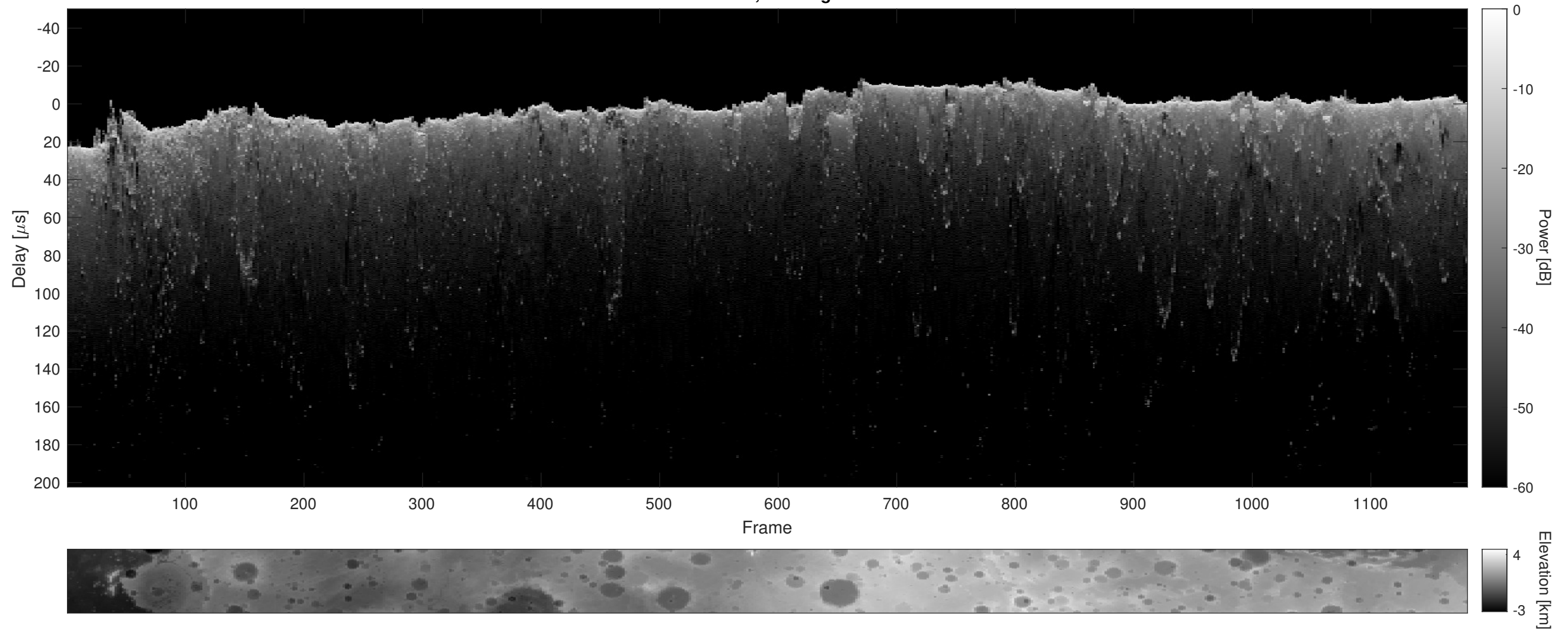
Orbit 9248, Cluttergram
