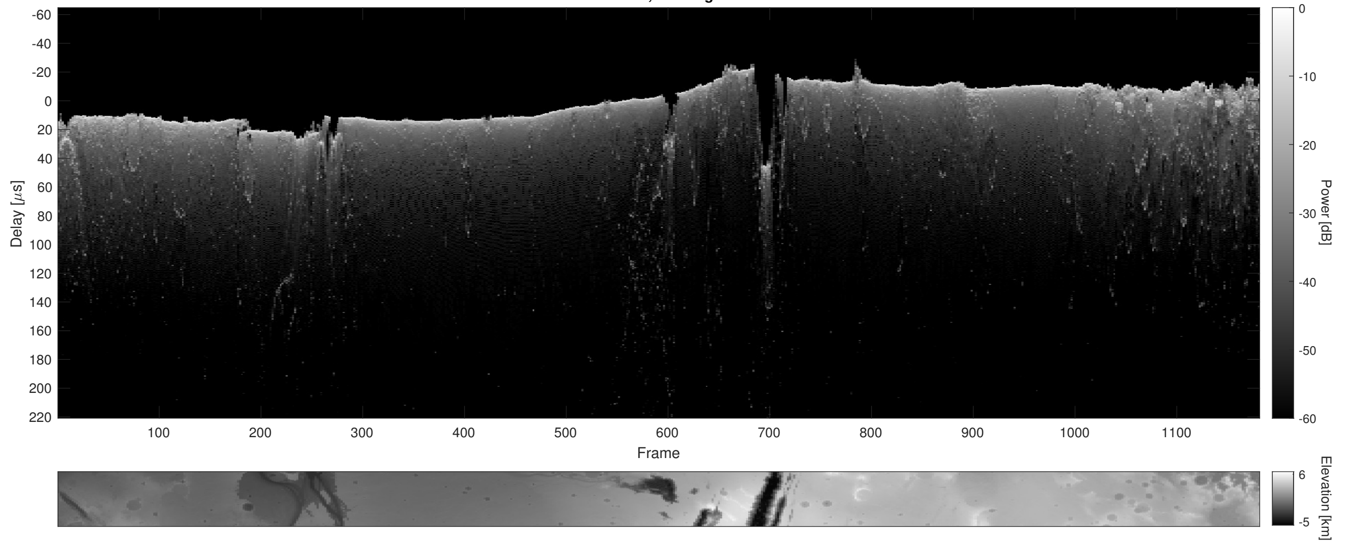
Orbit 9249, Cluttergram
