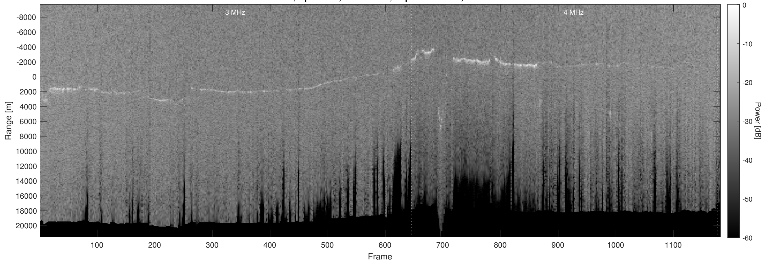
Orbit 9249, Optimized, No Window, Depth-Corrected, Channel 2
