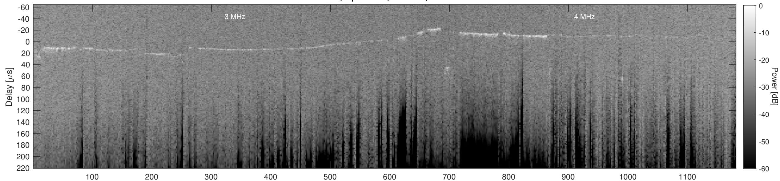
Orbit 9249, Cluttergram
