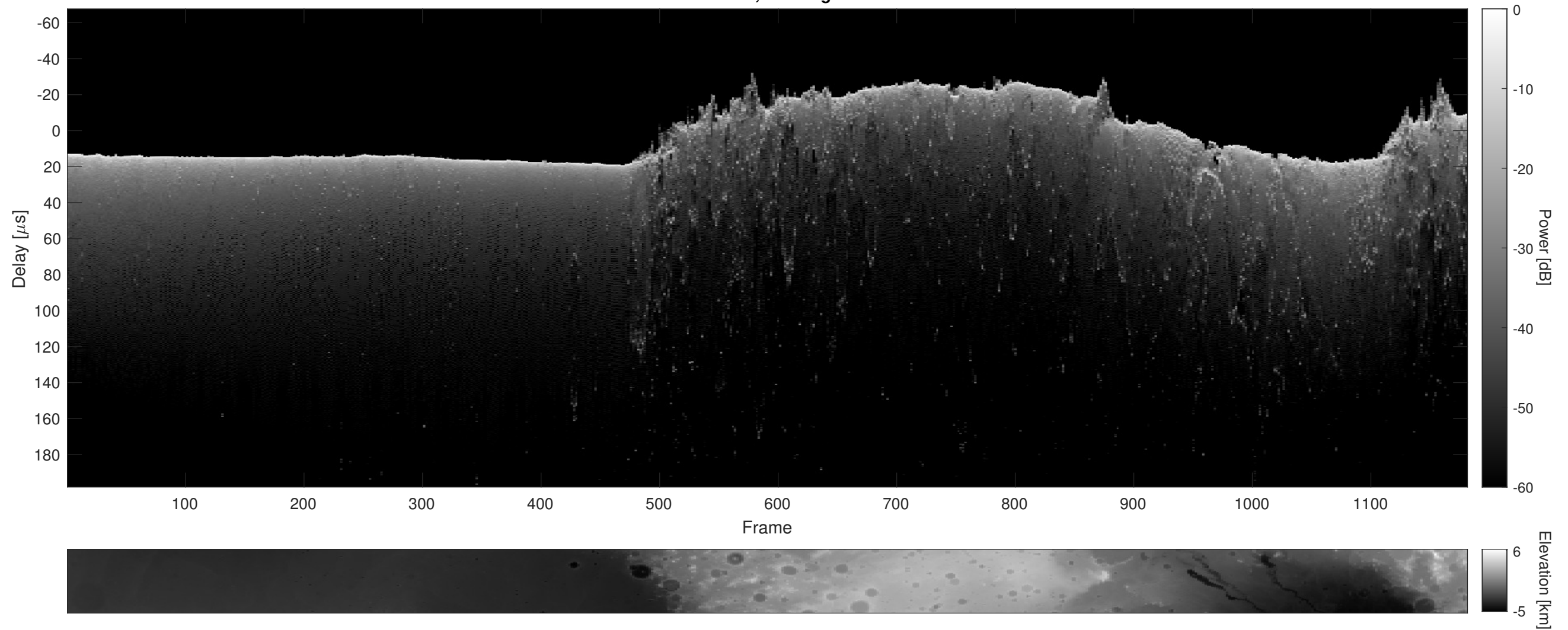
Orbit 9251, Cluttergram
