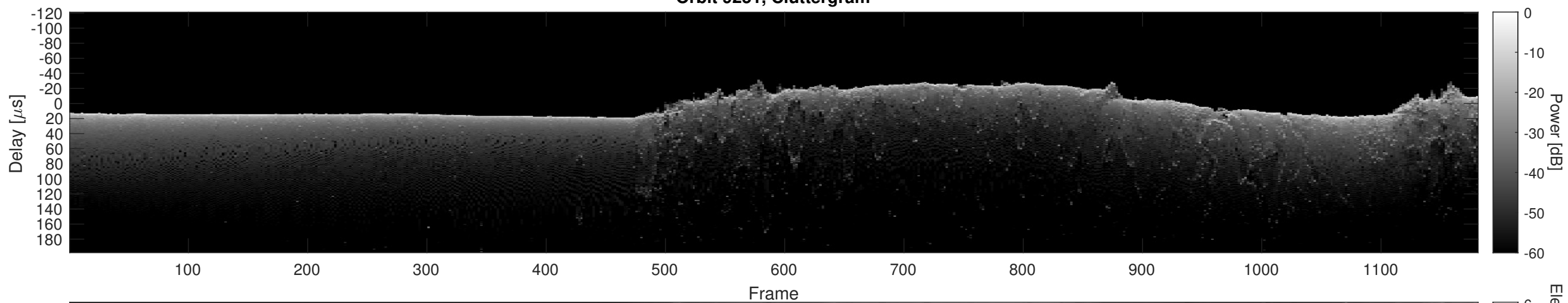
Orbit 9251, Cluttergram
