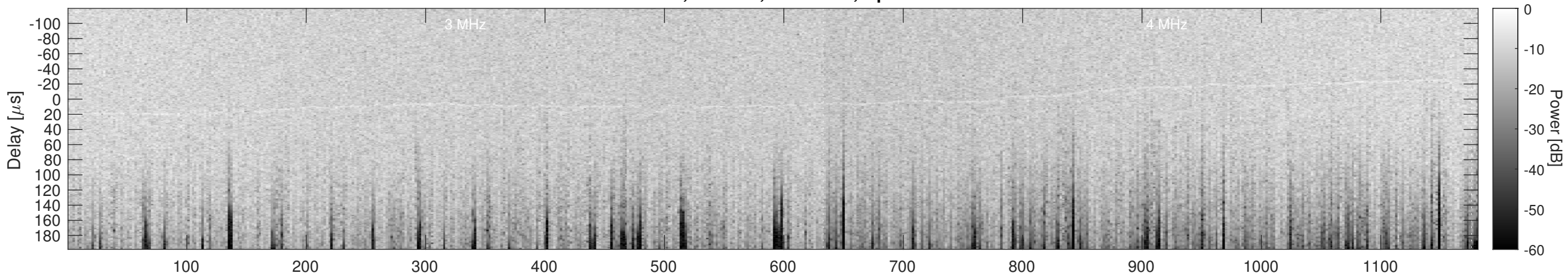
Orbit 9252, Cluttergram
