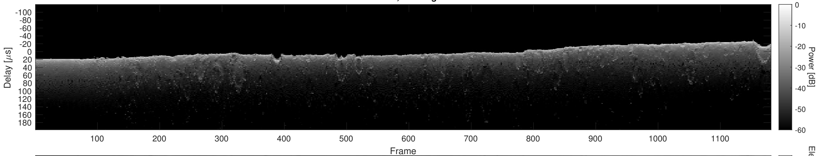
Orbit 9252, Cluttergram
