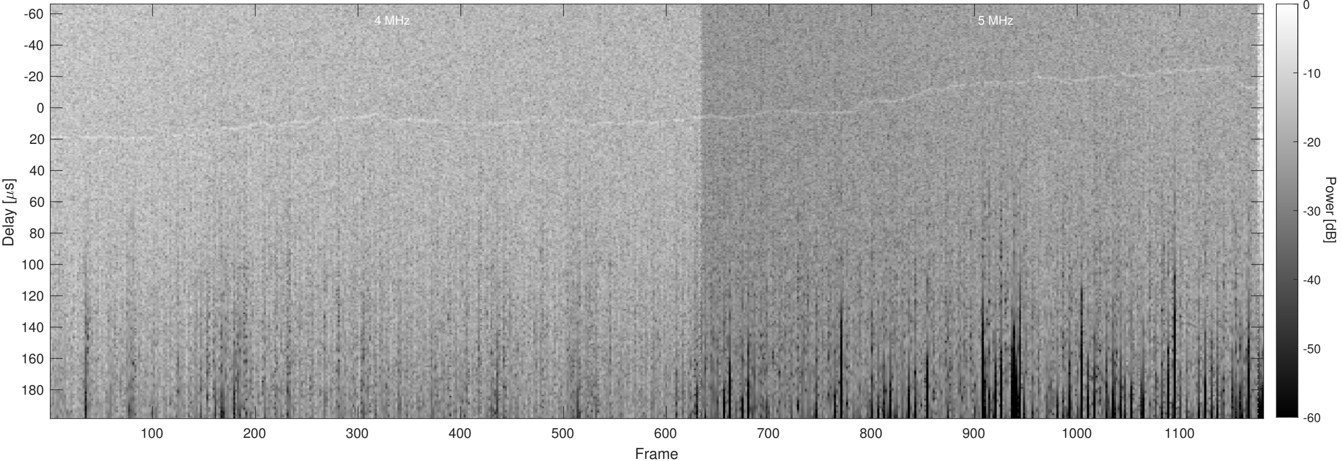
Orbit 9252, Optimized, No Window, Channel 2
