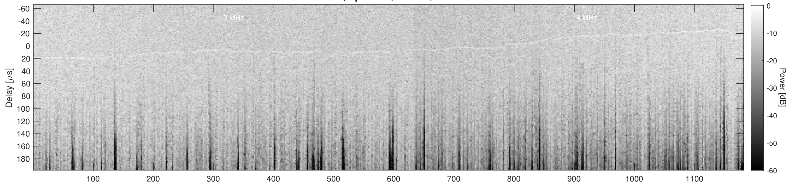
Orbit 9252, Cluttergram
