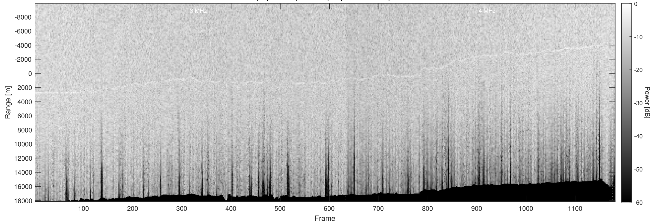
Orbit 9252, Optimized, Window, Depth-Corrected, Channel 2
