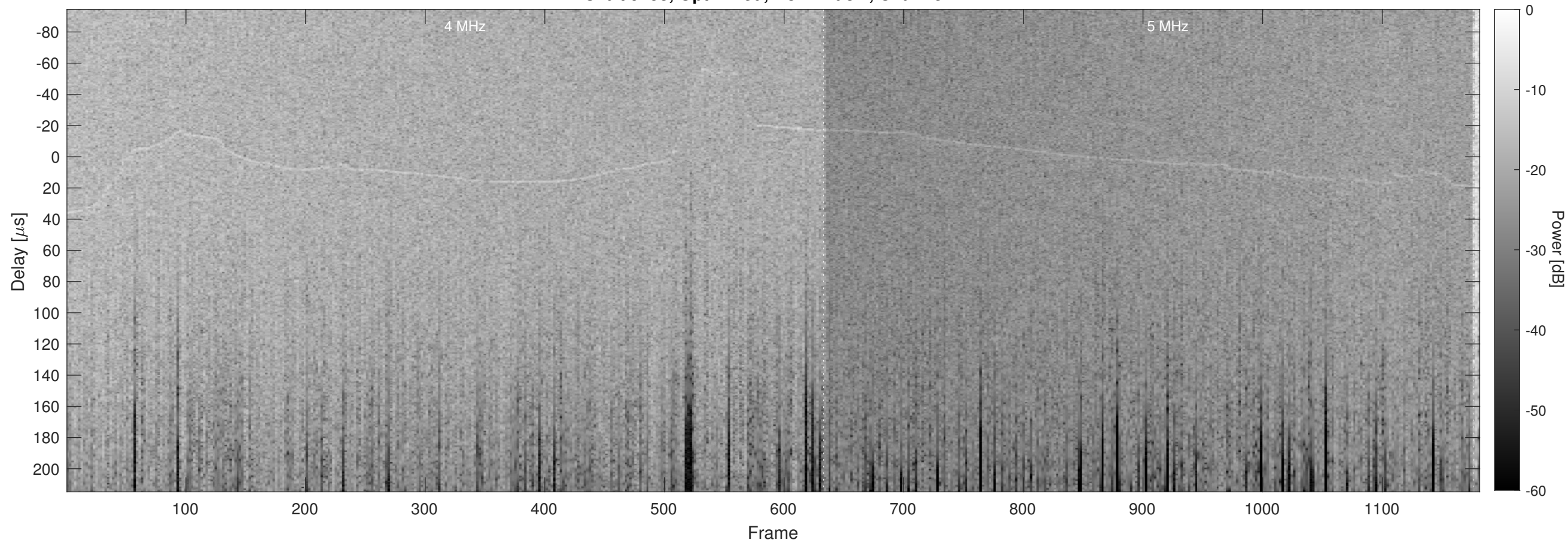
Orbit 9253, Optimized, No Window, Channel 2
