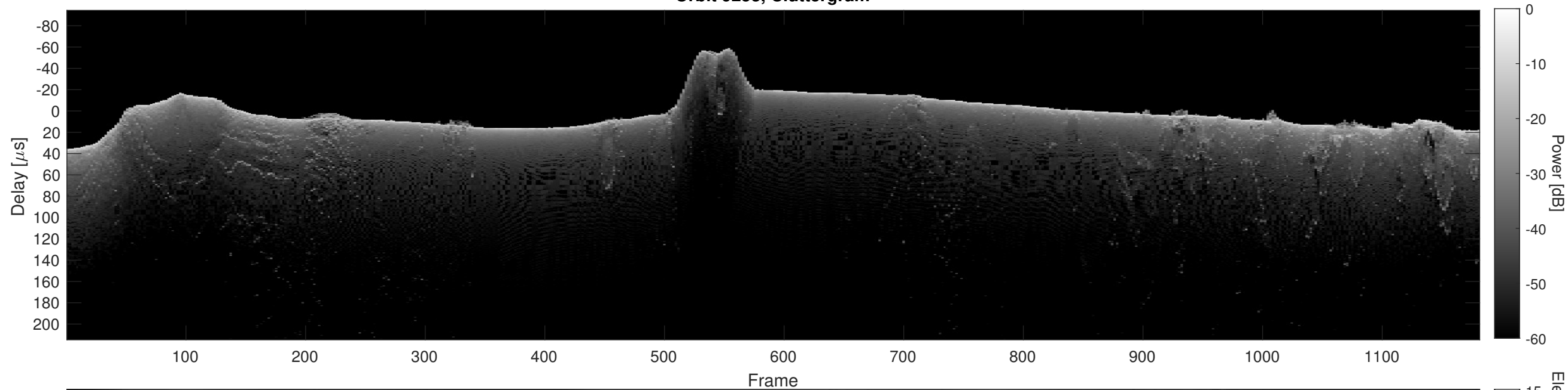
Orbit 9253, Cluttergram
