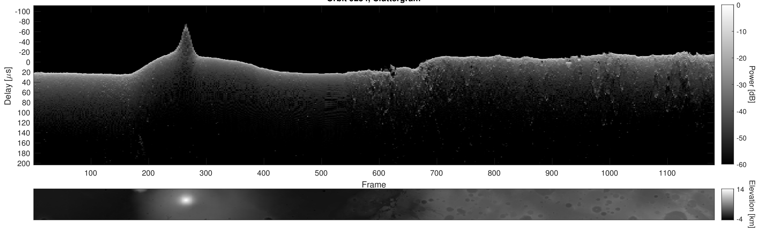
Orbit 9254, Cluttergram
