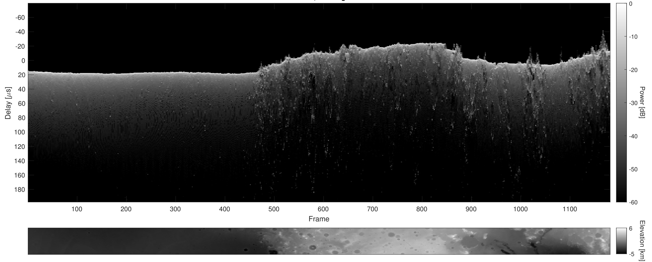
Orbit 9258, Cluttergram
