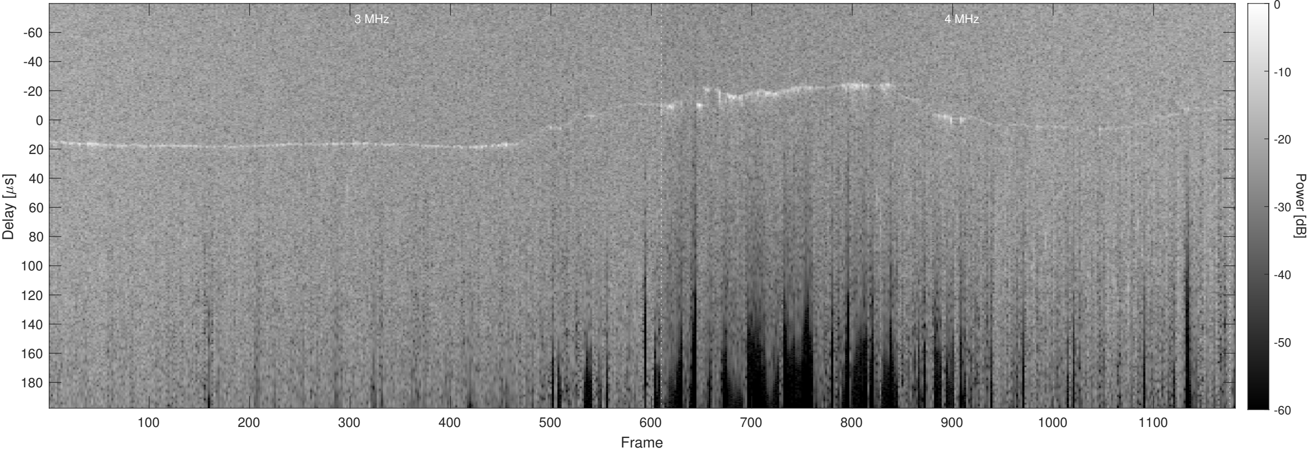
Orbit 9258, Optimized, No Window, Channel 2
