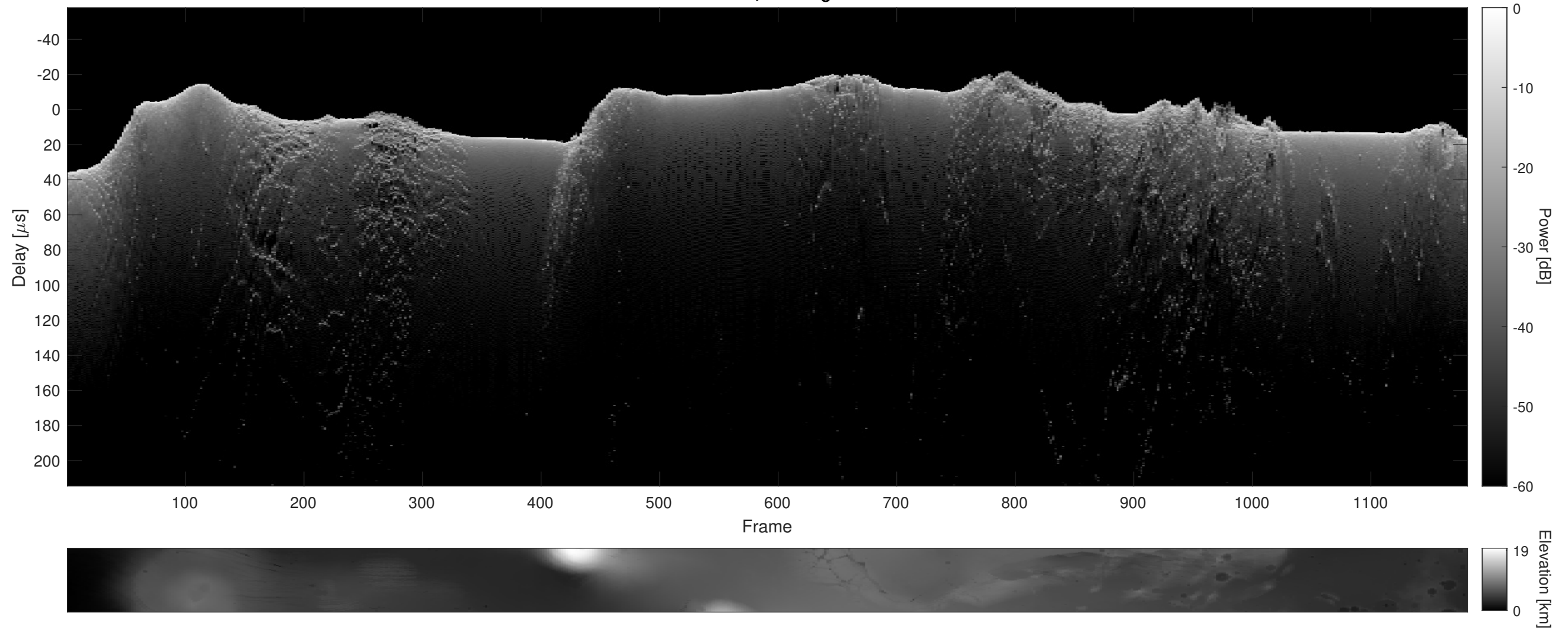
Orbit 9260, Cluttergram
