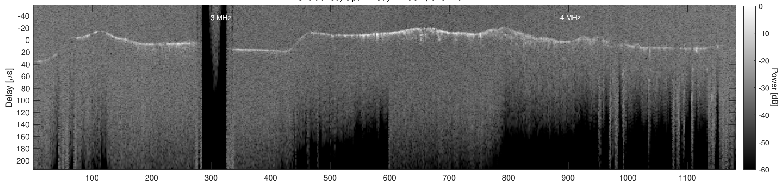
Orbit 9260, Cluttergram
