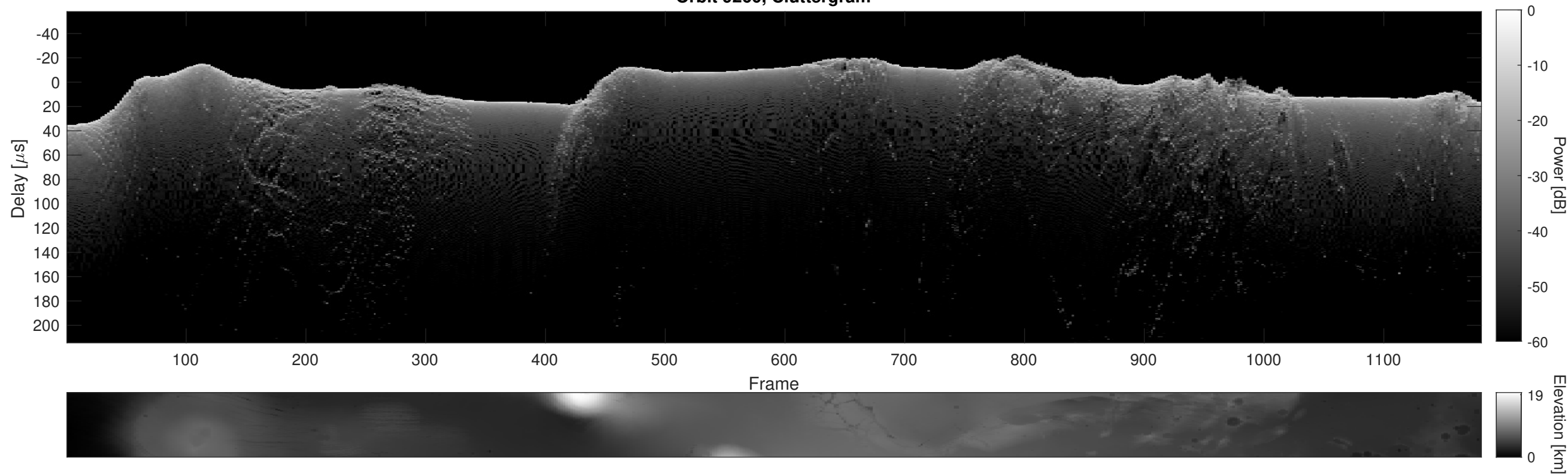
Orbit 9260, Cluttergram
