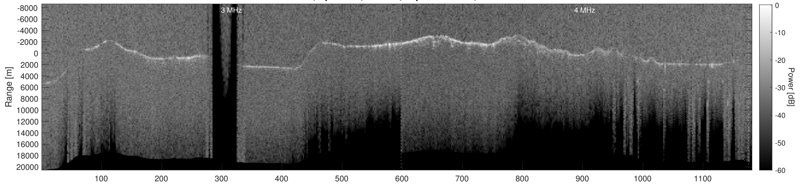
Orbit 9260, Depth-Corrected Cluttergram
