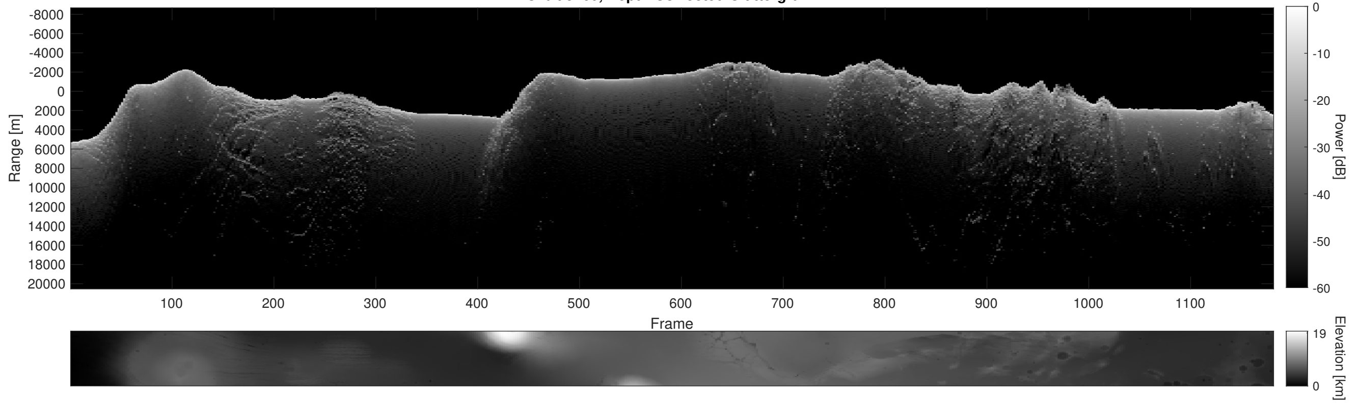
Orbit 9260, Depth-Corrected Cluttergram
