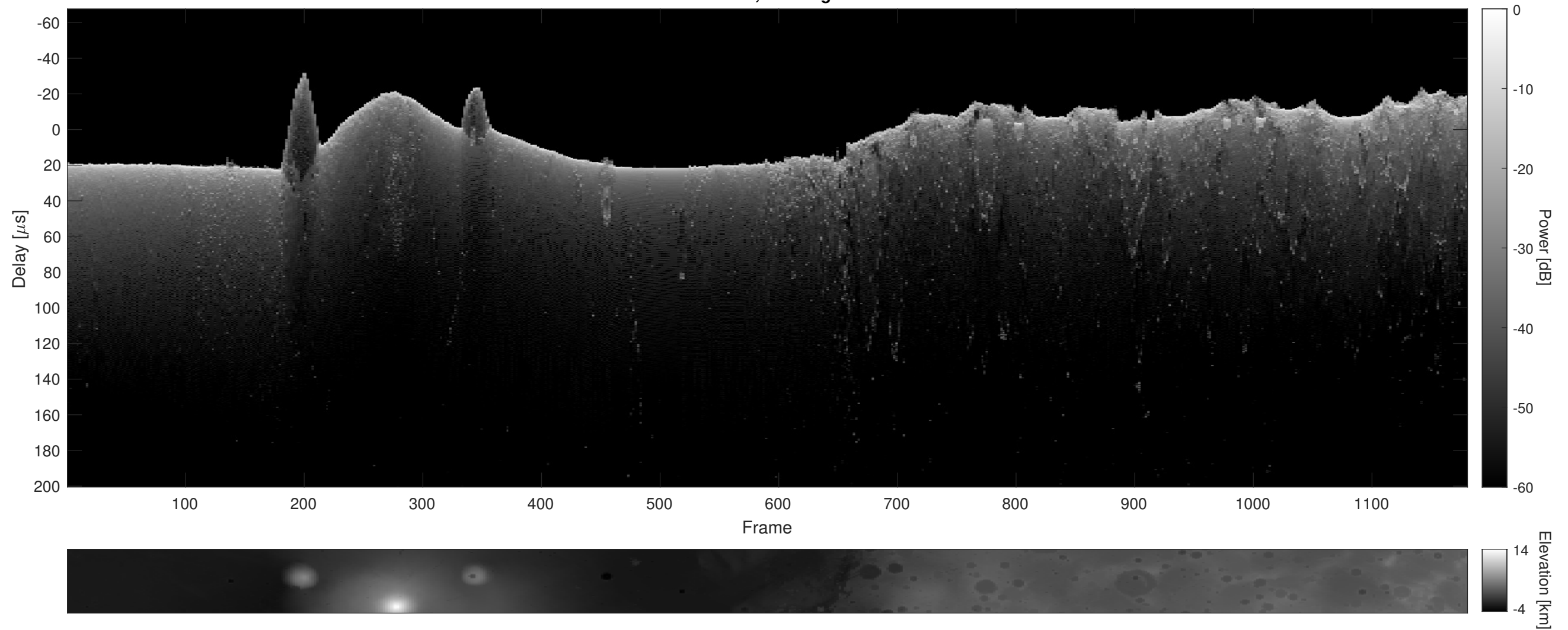
Orbit 9261, Cluttergram
