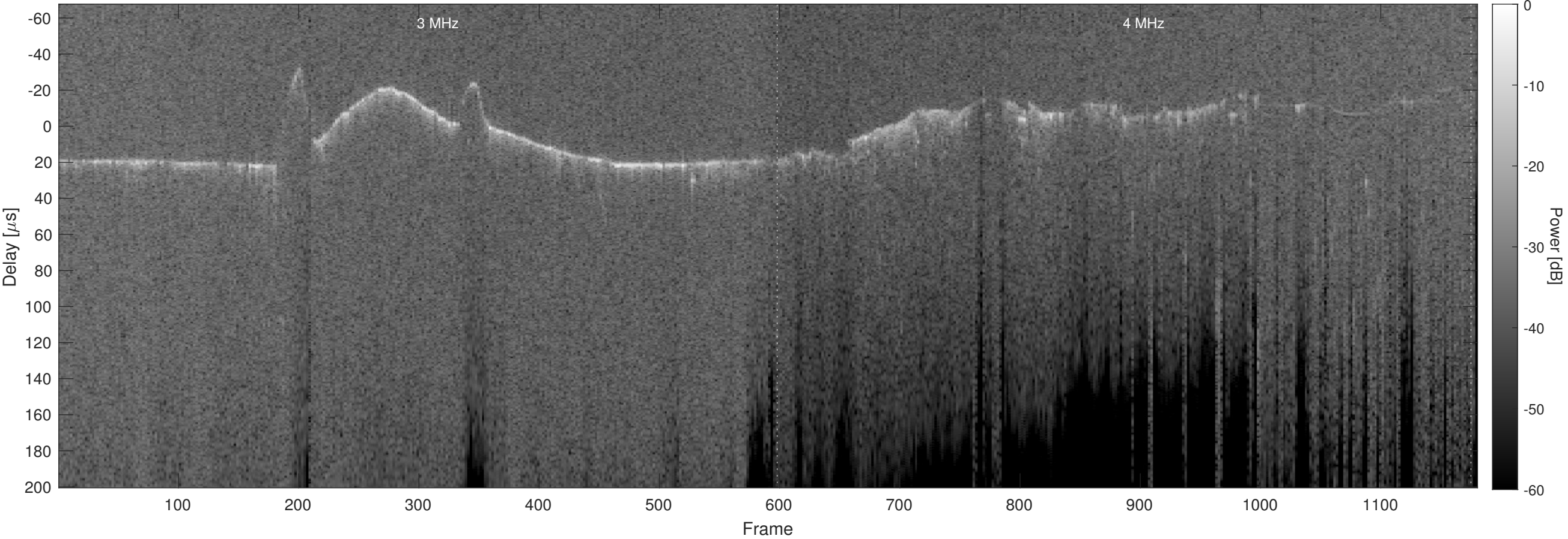
Orbit 9261, Optimized, No Window, Channel 2
