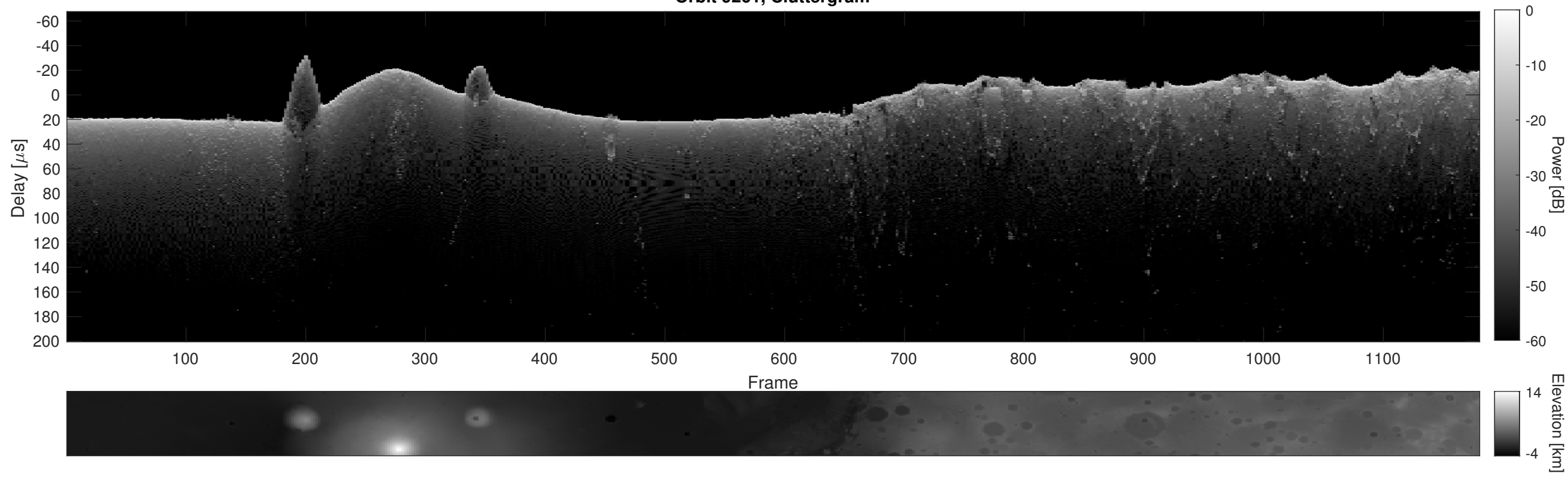
Orbit 9261, Cluttergram
