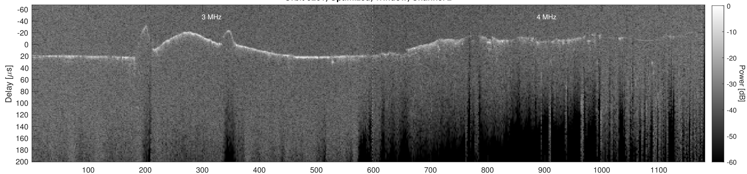
Orbit 9261, Cluttergram
