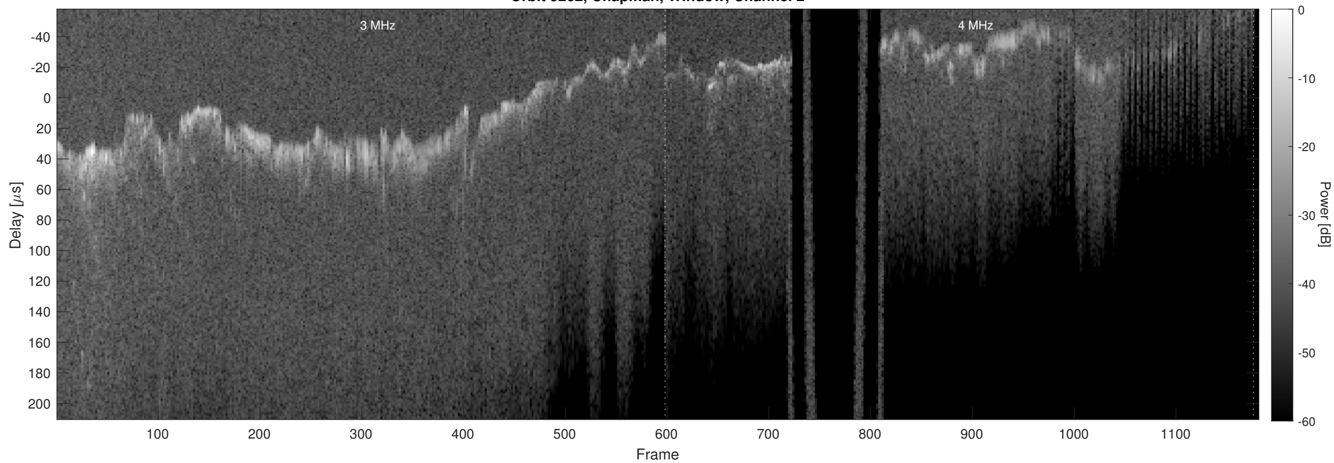
Orbit 9262, Chapman, Window, Channel 2
