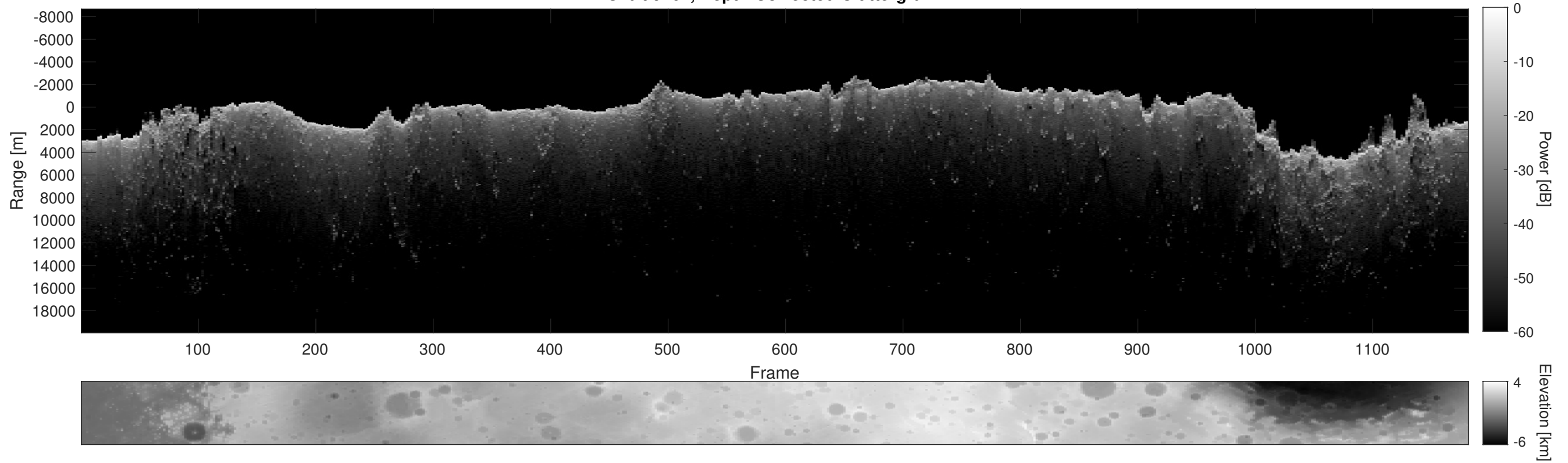
Orbit 9262, Depth-Corrected Cluttergram
