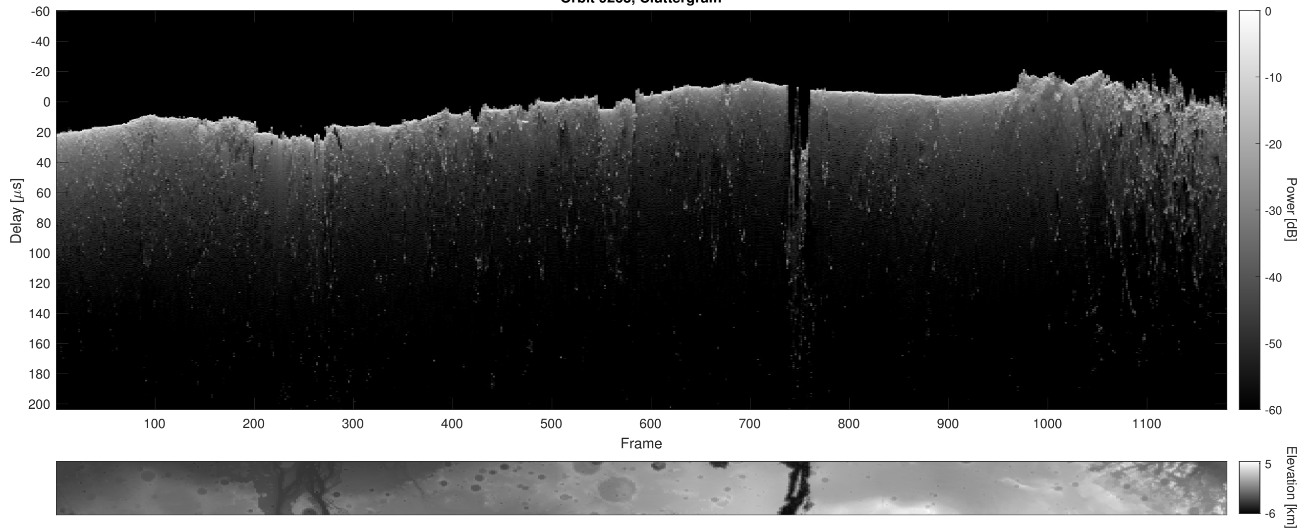
Orbit 9263, Cluttergram
