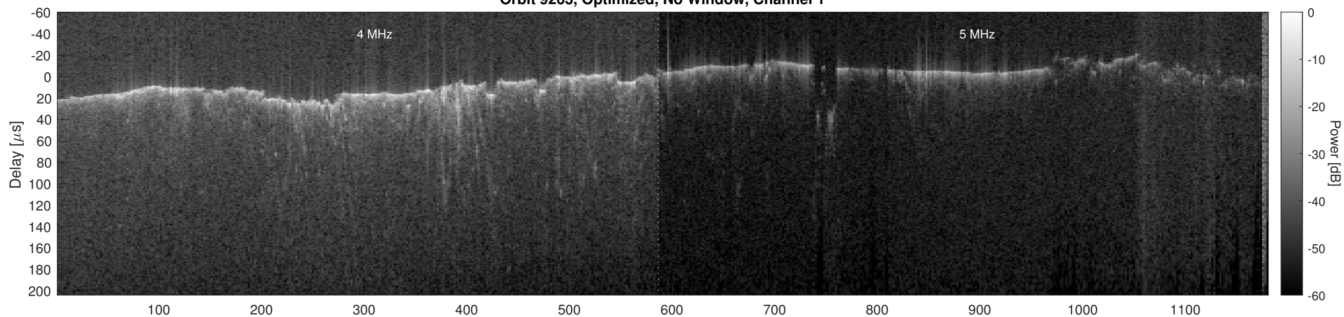
Orbit 9263, Optimized, No Window, Channel 2
