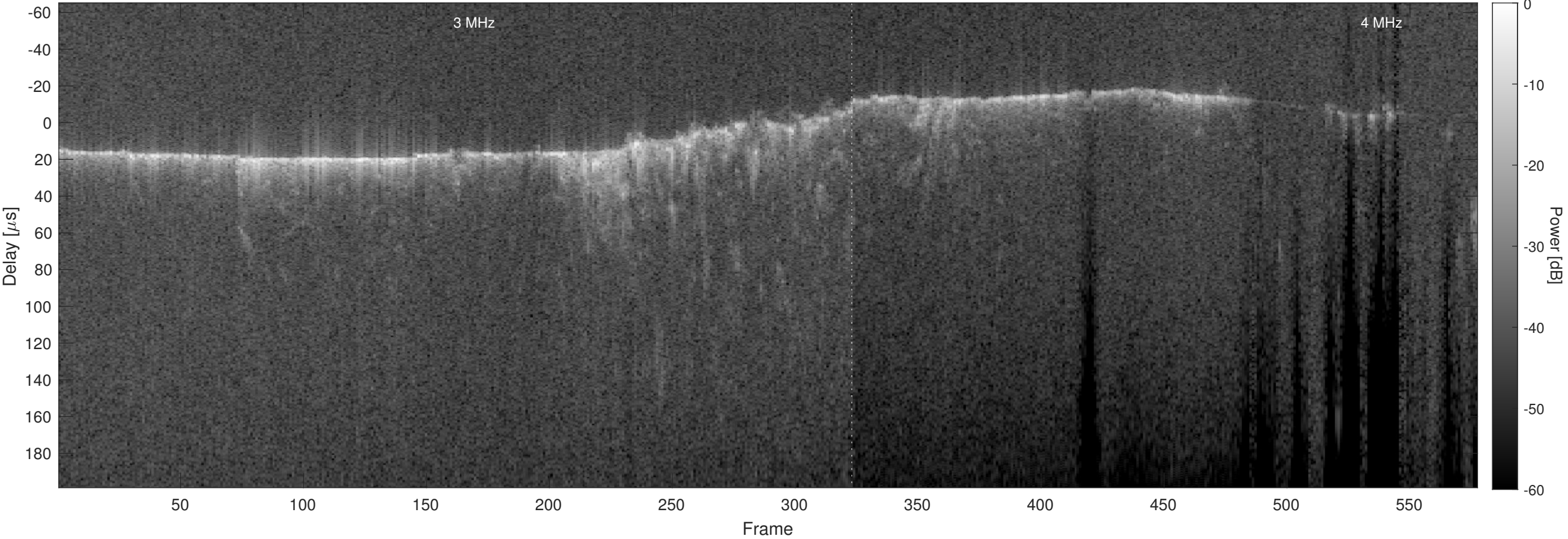
Orbit 9265, Optimized, No Window, Channel 2
