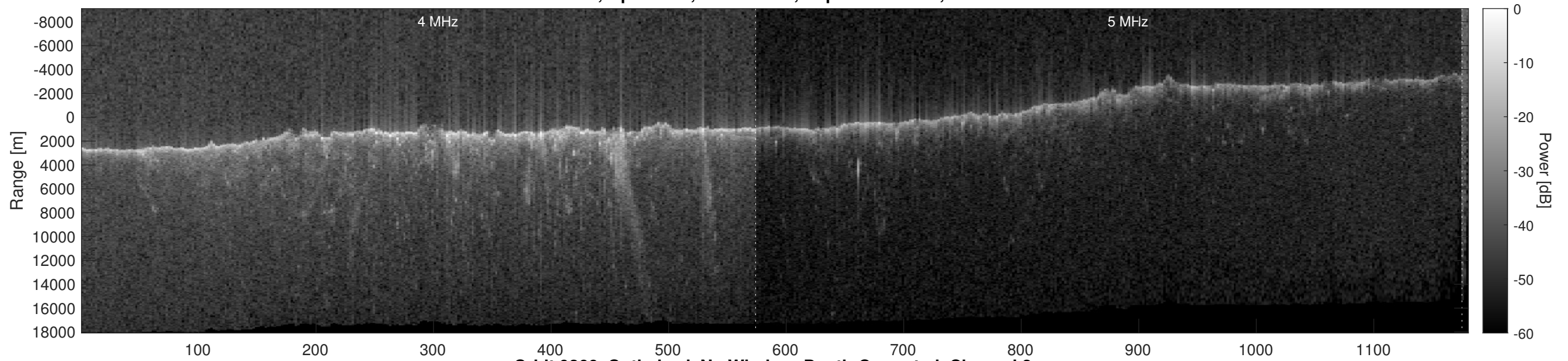
Orbit 9266, Optimized, No Window, Depth-Corrected, Channel 2
