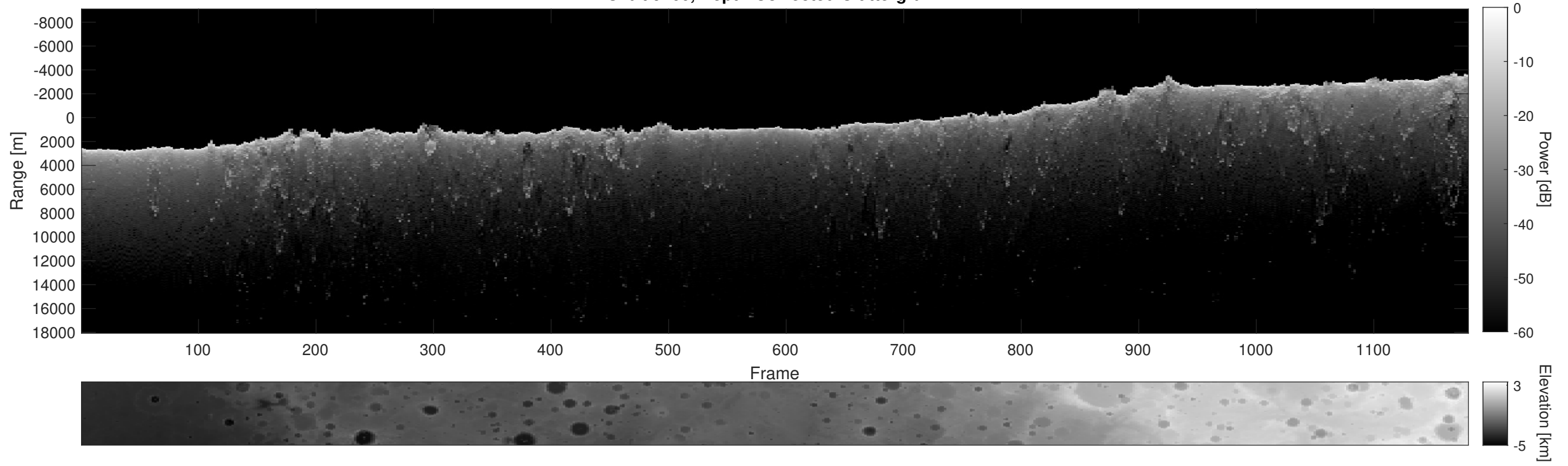
Orbit 9266, Depth-Corrected Cluttergram
