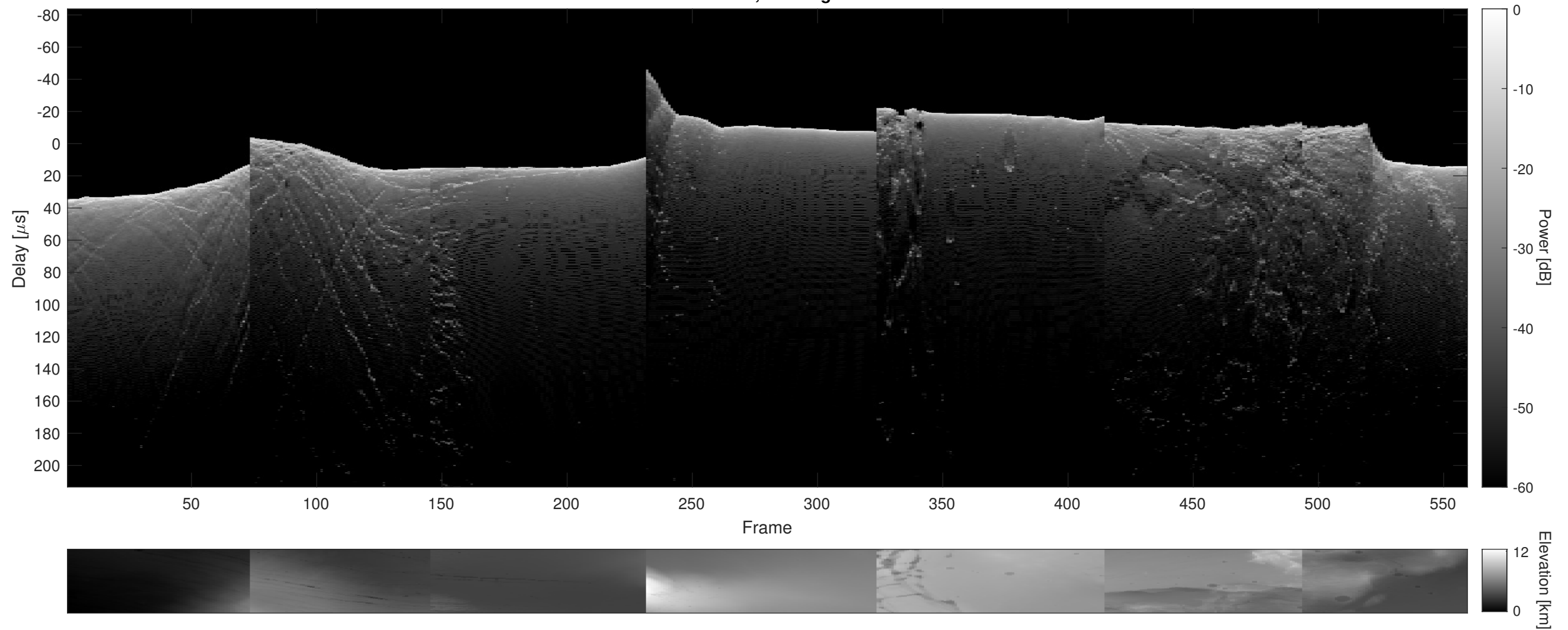
Orbit 9267, Cluttergram
