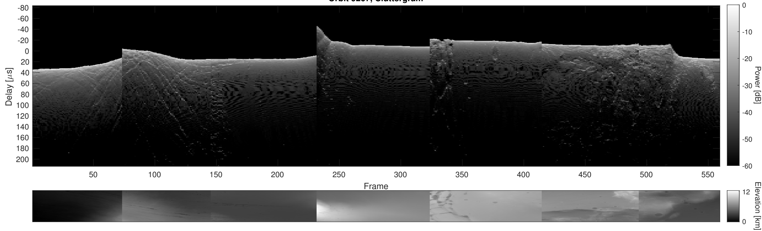
Orbit 9267, Cluttergram
