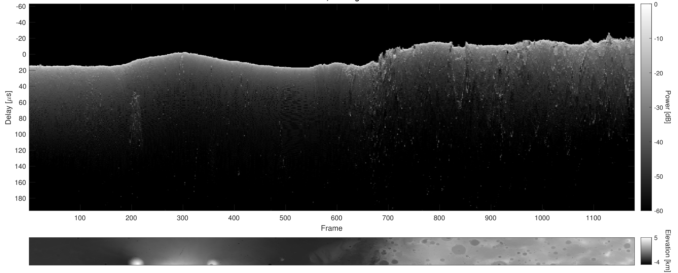
Orbit 9268, Cluttergram
