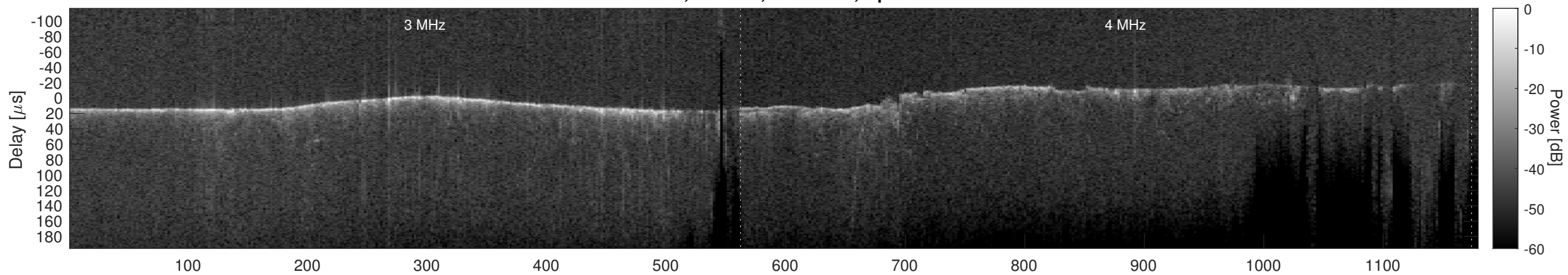
Orbit 9268, Cluttergram
