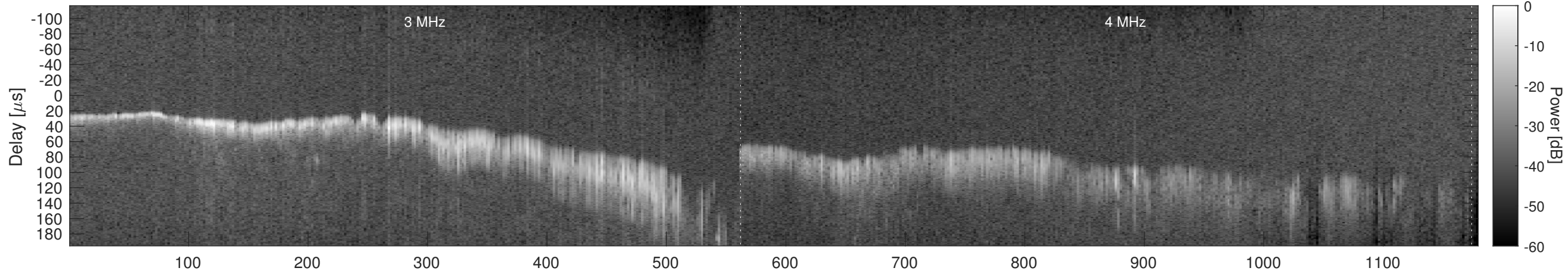
Orbit 9268, Window, Channel 2, Chapman
