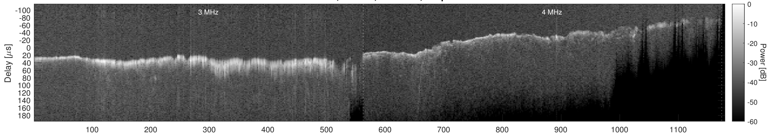
Orbit 9268, Window, Channel 2, Optimized
