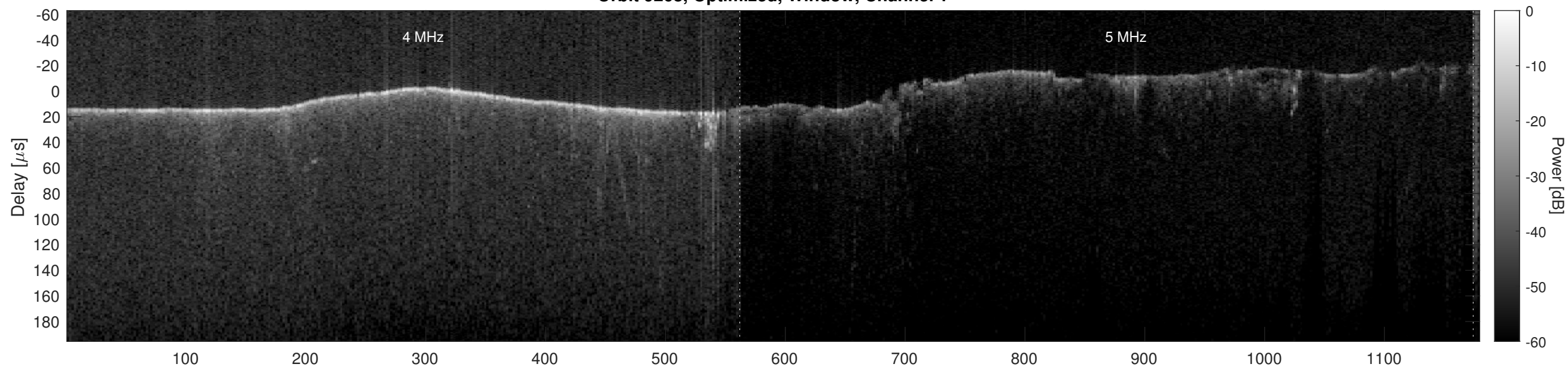
Orbit 9268, Optimized, Window, Channel 2
