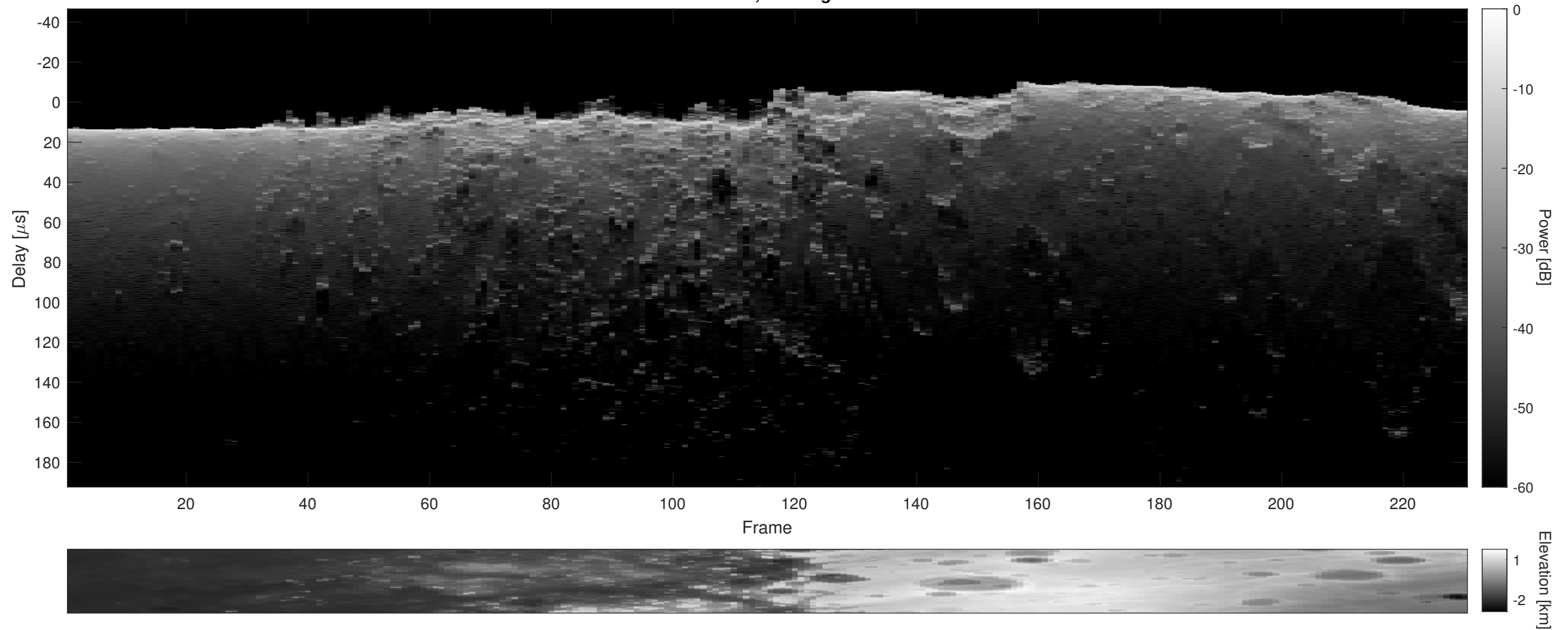
Orbit 9269, Cluttergram
