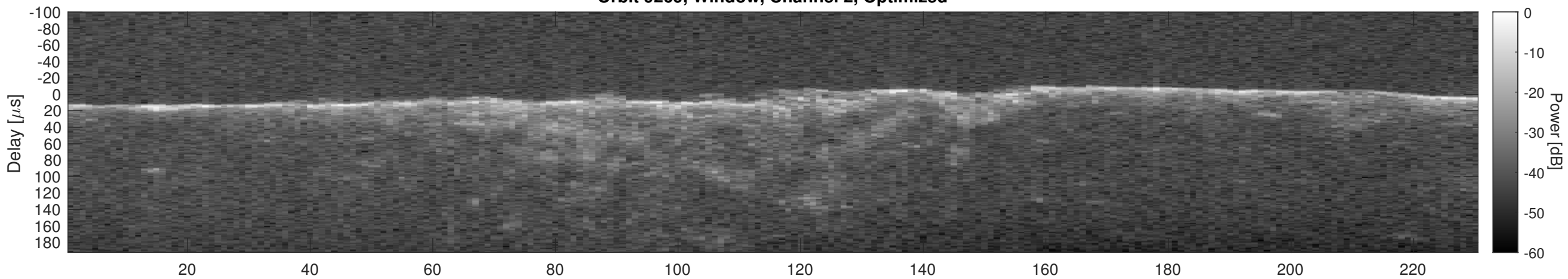
Orbit 9269, Cluttergram
