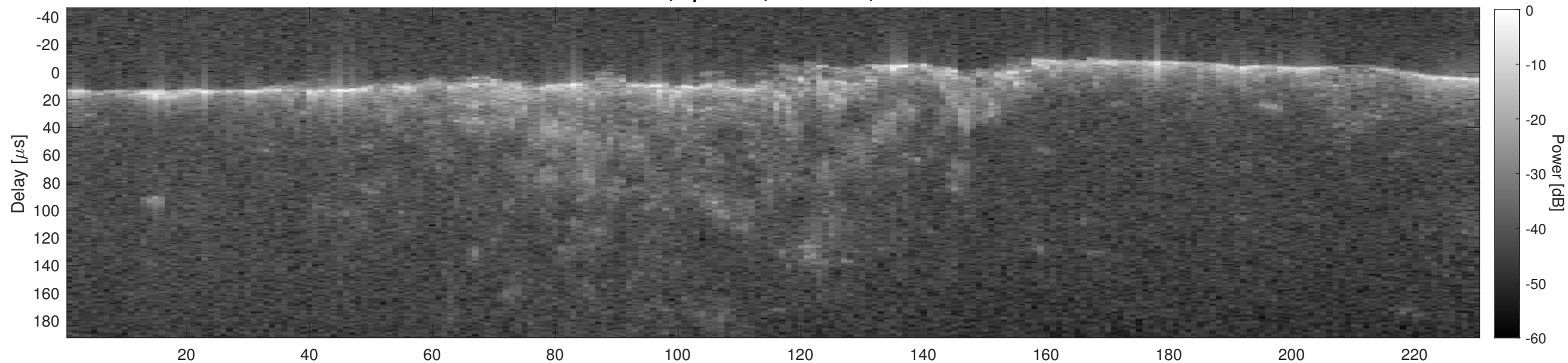
Orbit 9269, Cluttergram
